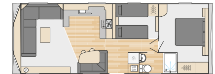
32' x 12' - 2 Bedroom
